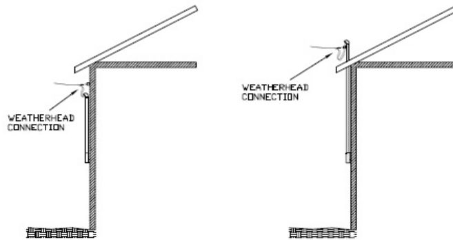
~ OVERHEAD SERVICE ~
